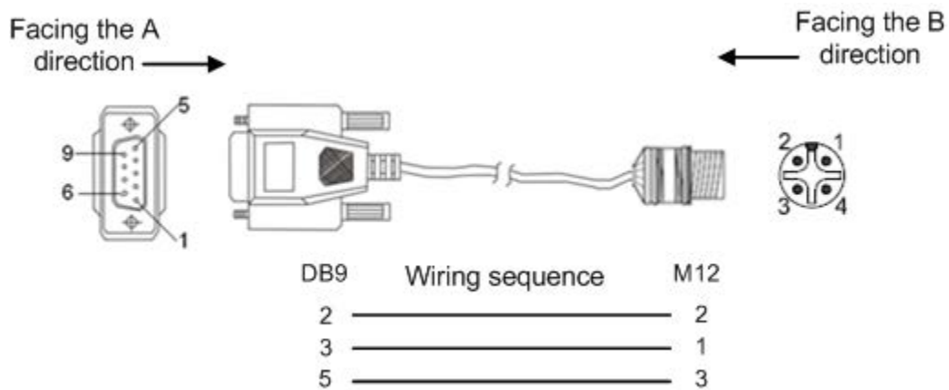
Figure 13 Wiring Sequence M12-DB9 Console Cable
