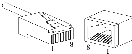
Figure 10 RJ45 Port
