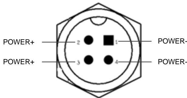
Figure 18 External Power Port (male)
