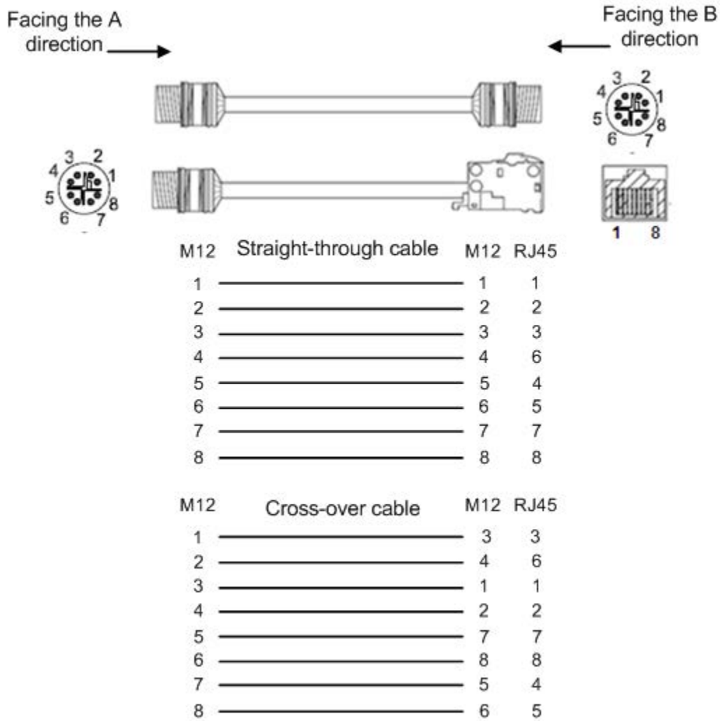
Figure 11 Connection Using Straight-through/Cross-over Cable
