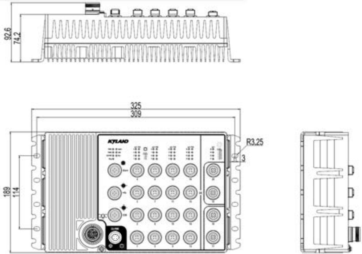
Figure 3 Aquam8120/8620 Series Dimensions (unit: mm)
