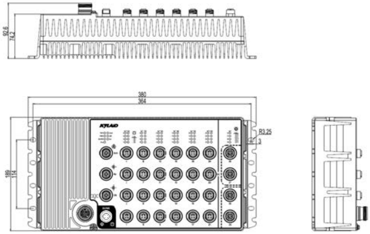
Figure 4 Aquam8128/8628 Series Dimensions (unit: mm)
