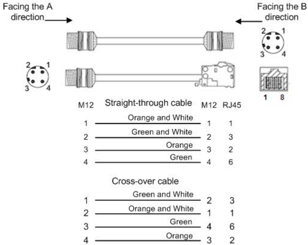
Figure 8 Connection Using Straight-through/Cross-over Cable
