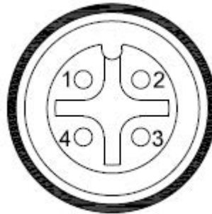
Figure 12 Console Port (female)
