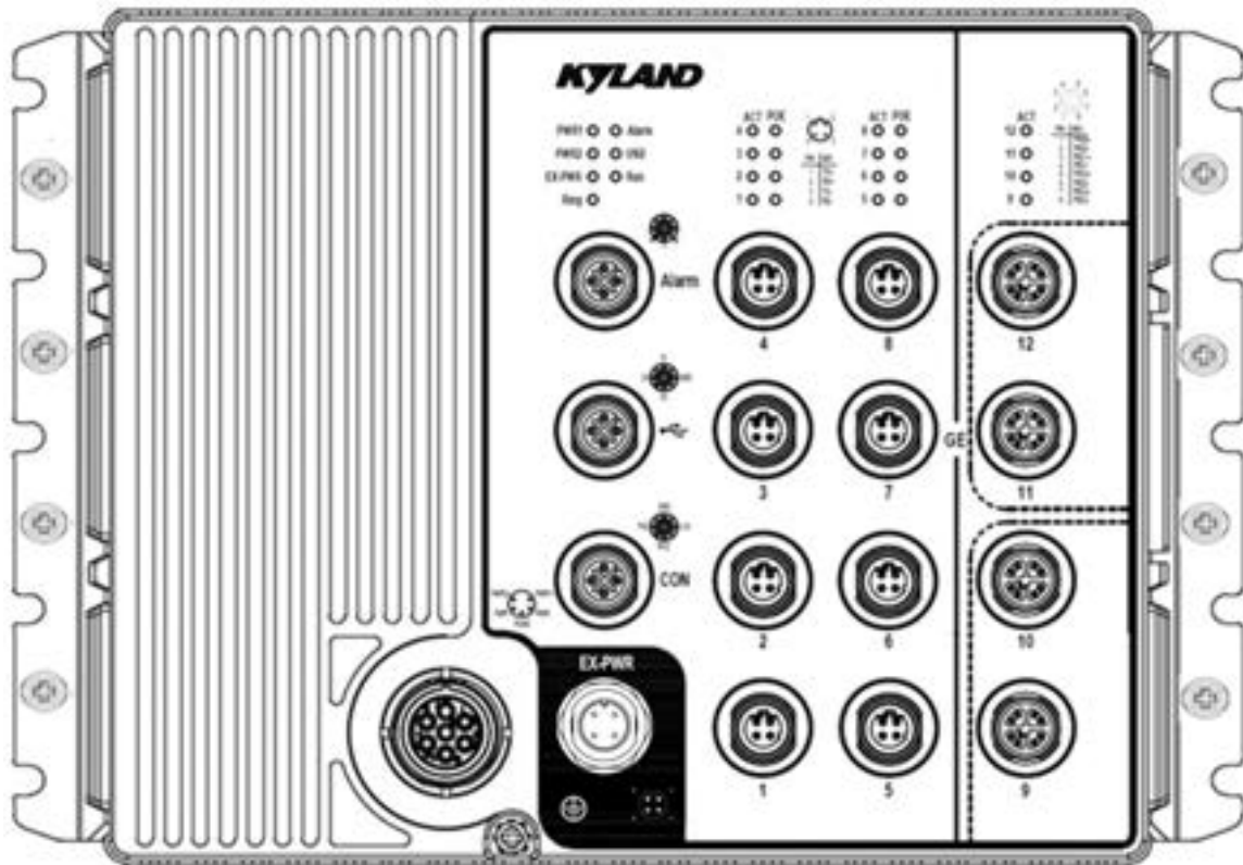
Figure 5 Panel Mounting
