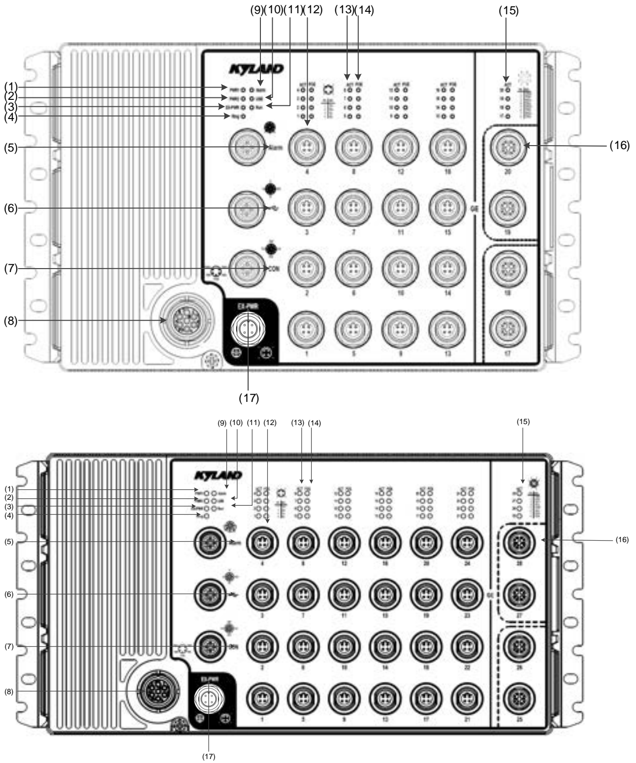
Figure 1 Front Panel
