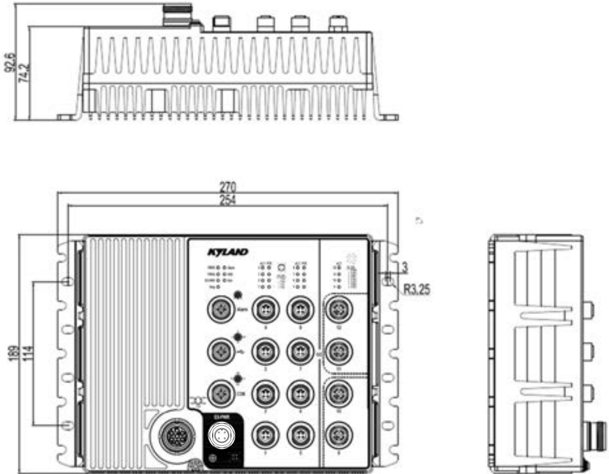
Figure 2 Aquam8112/8612 Series Dimensions (unit: mm)
