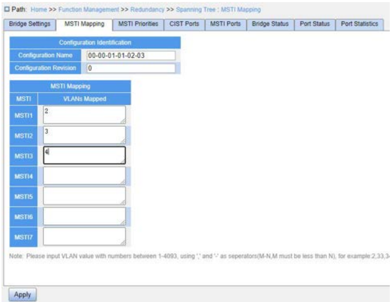
Figure 148 Configure MSTI Mapping
