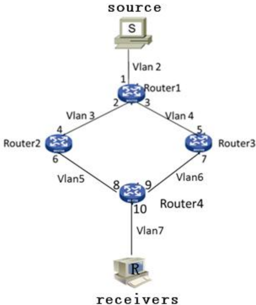
Figure 221 PIM DM Example
