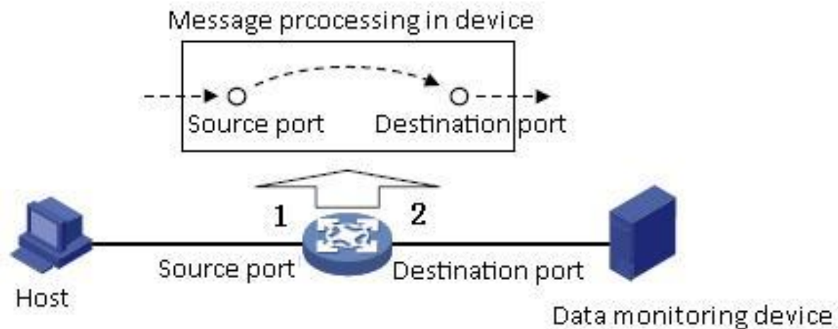
Figure 280 Port Mirroring Example
