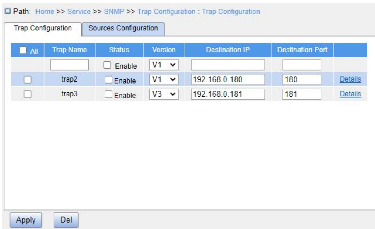
Figure 49 Configure Trap
