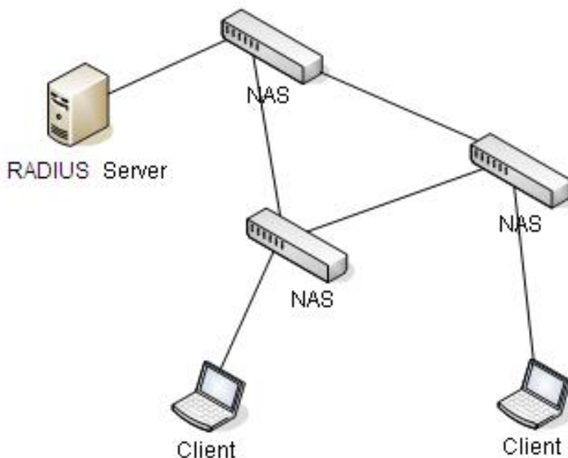
Figure 65 RADIUS Structure
