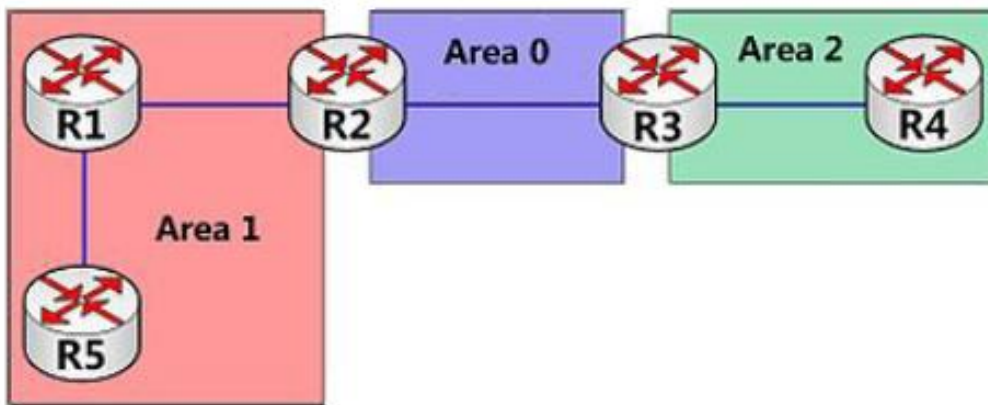
Figure 238 Area Partition
