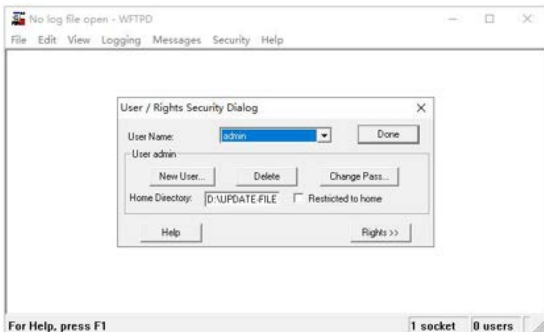
Figure 30 File Location
