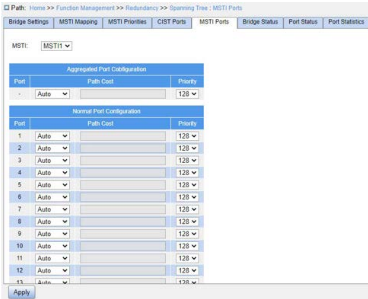
Figure 151 Select MSTI
