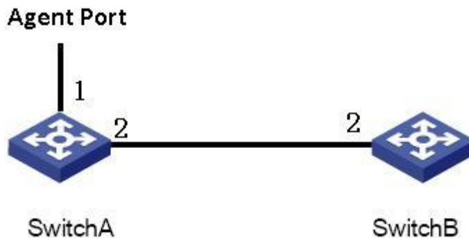
Figure 209 GMRP Networking
