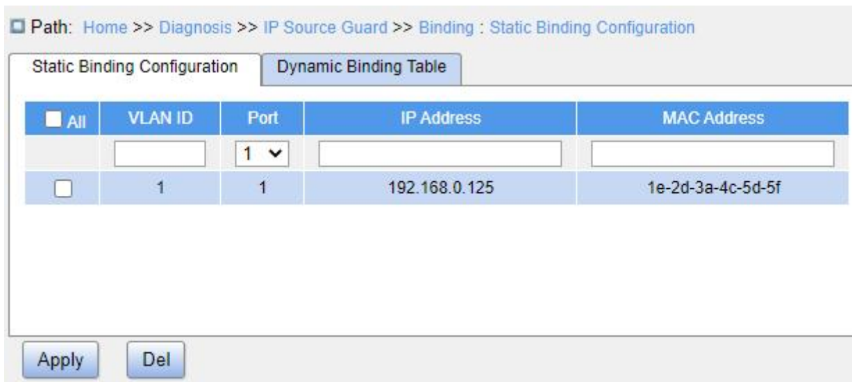
Figure 290 Cofnigure Static Binding
