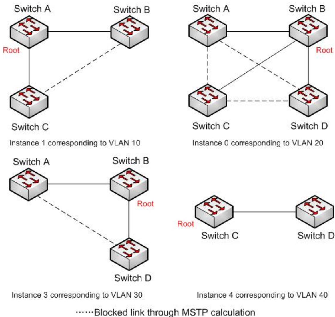
Figure 156 Spanning Tree Instance of Each VLAN
