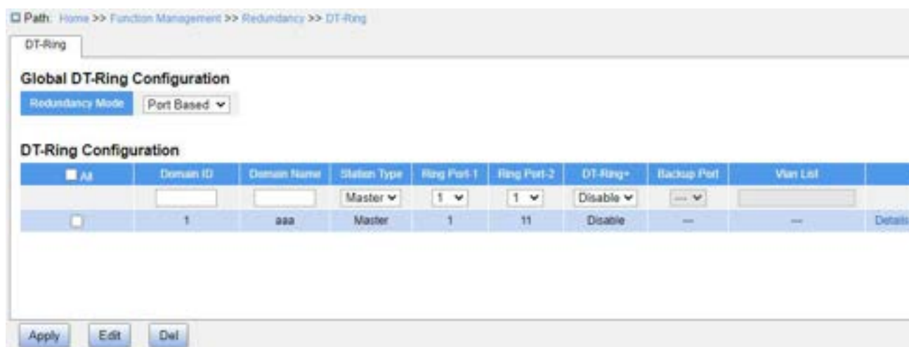
Figure 122 DT-Ring-Port Configuration
