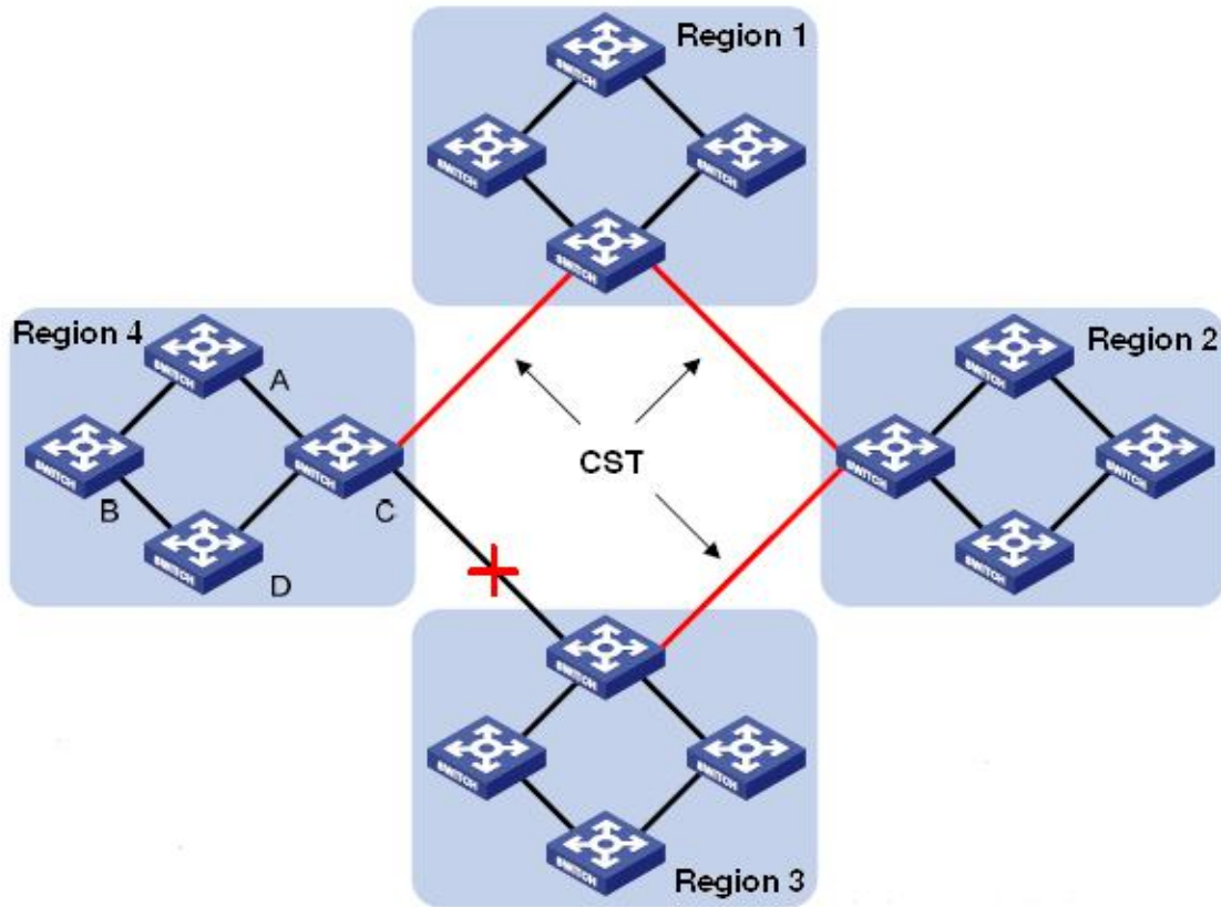
Figure 143 MSTP Concepts
