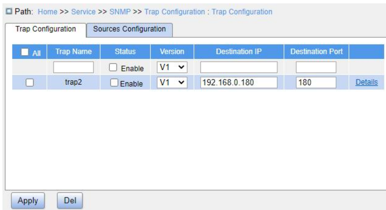
Figure 44 Configure Trap
