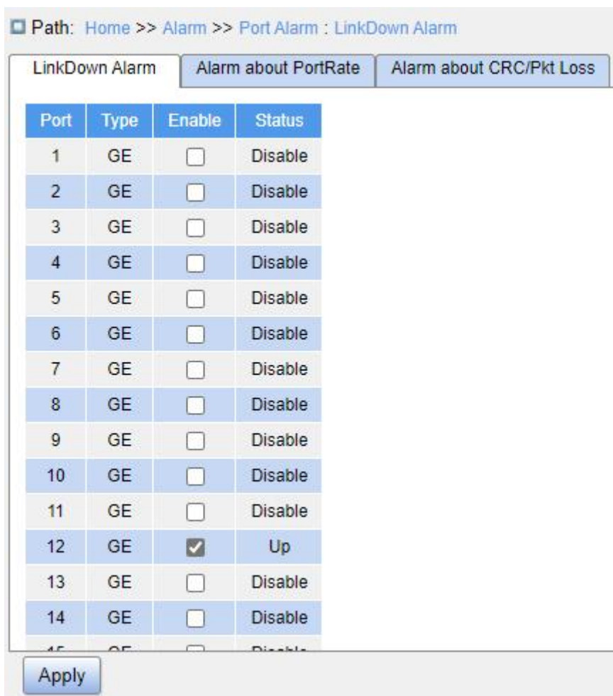
Figure 82 Port Alarm
