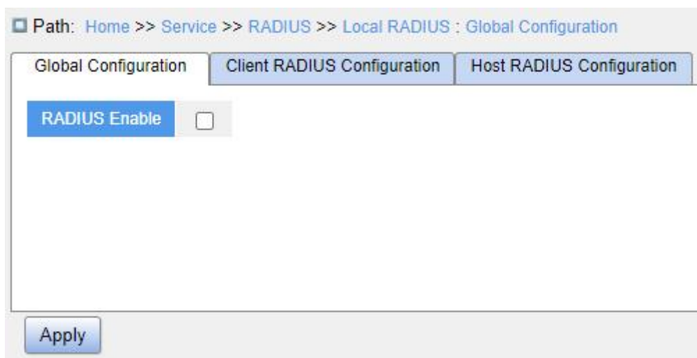
Figure 67 Global Configuration
