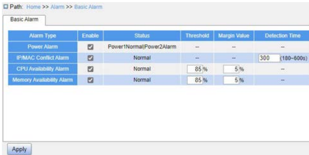
Figure 81 Basic Alarm
