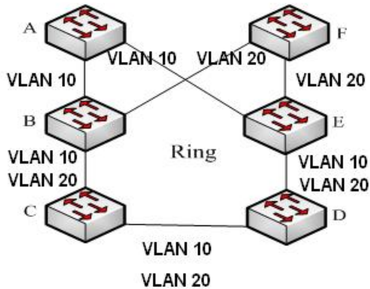
Figure 119 DT-Ring-VLAN
