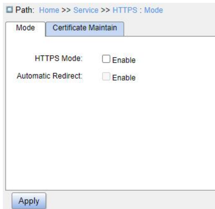
Figure 38 Enable HTTPS
