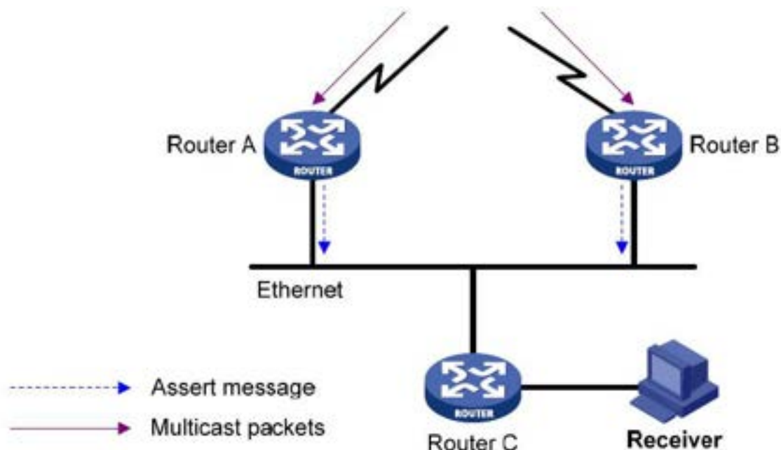
Figure 210 Assert mechanism diagram
