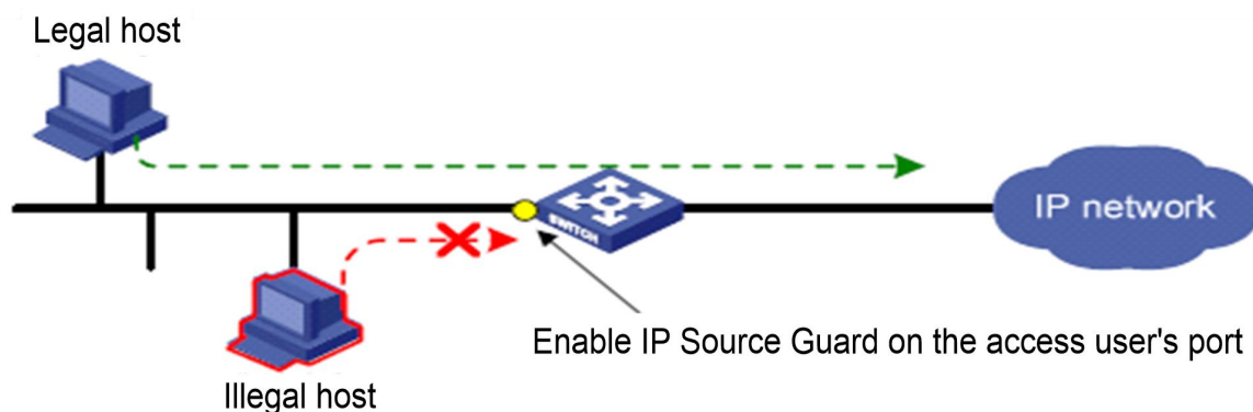
Figure 287 IP Source Guard Function Diagram
