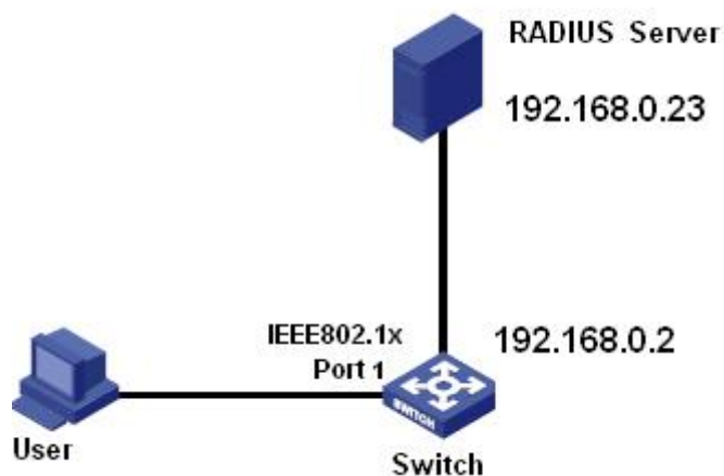
Figure 70 RADIUS Authentication Configuration Example
