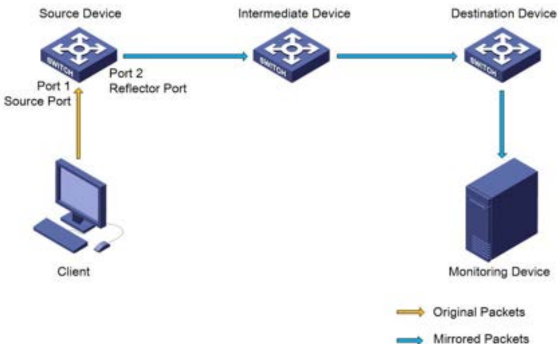
Figure 277 Remote Port Mirroring
