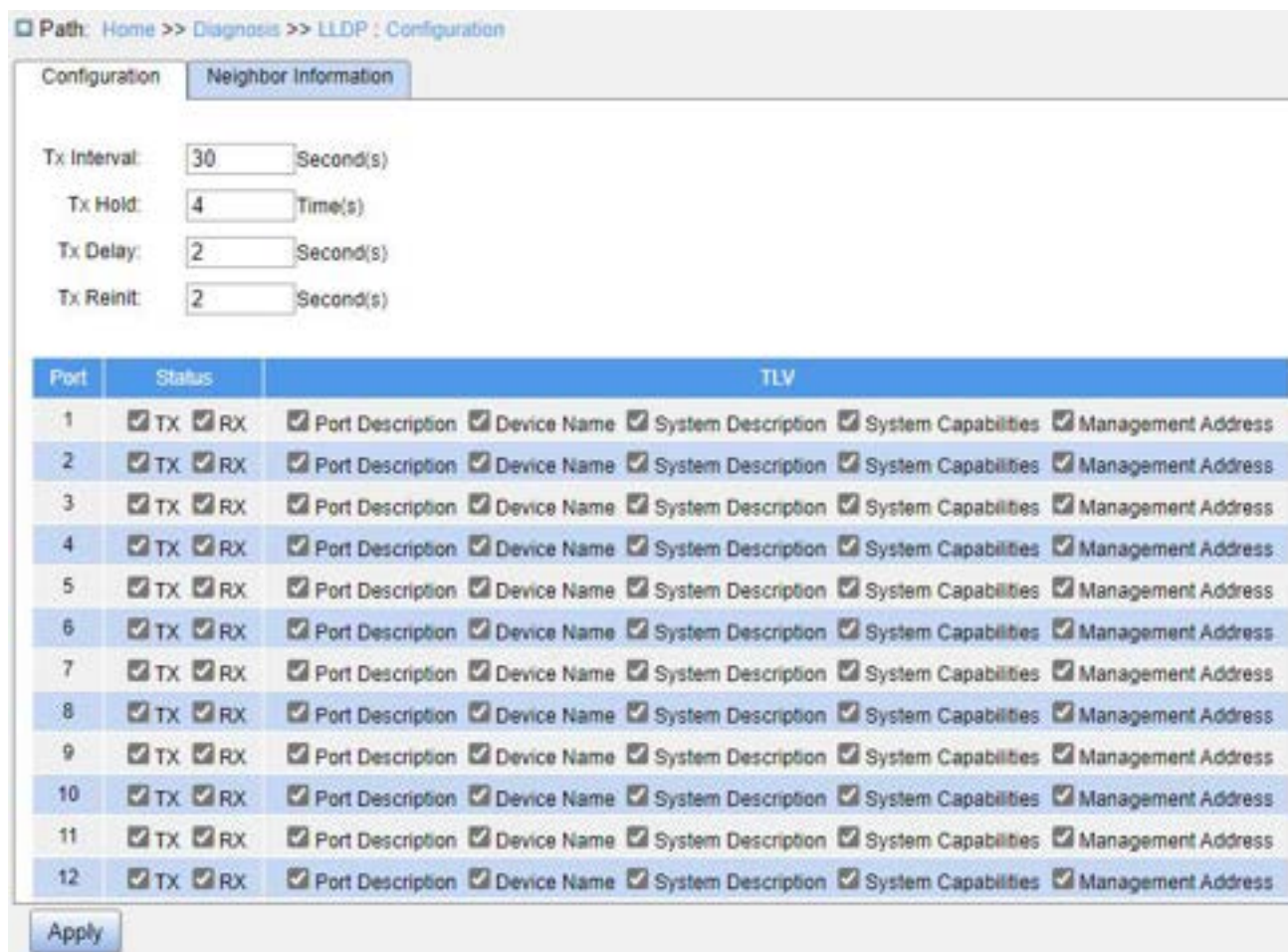
Figure 281 Configure LLDP
