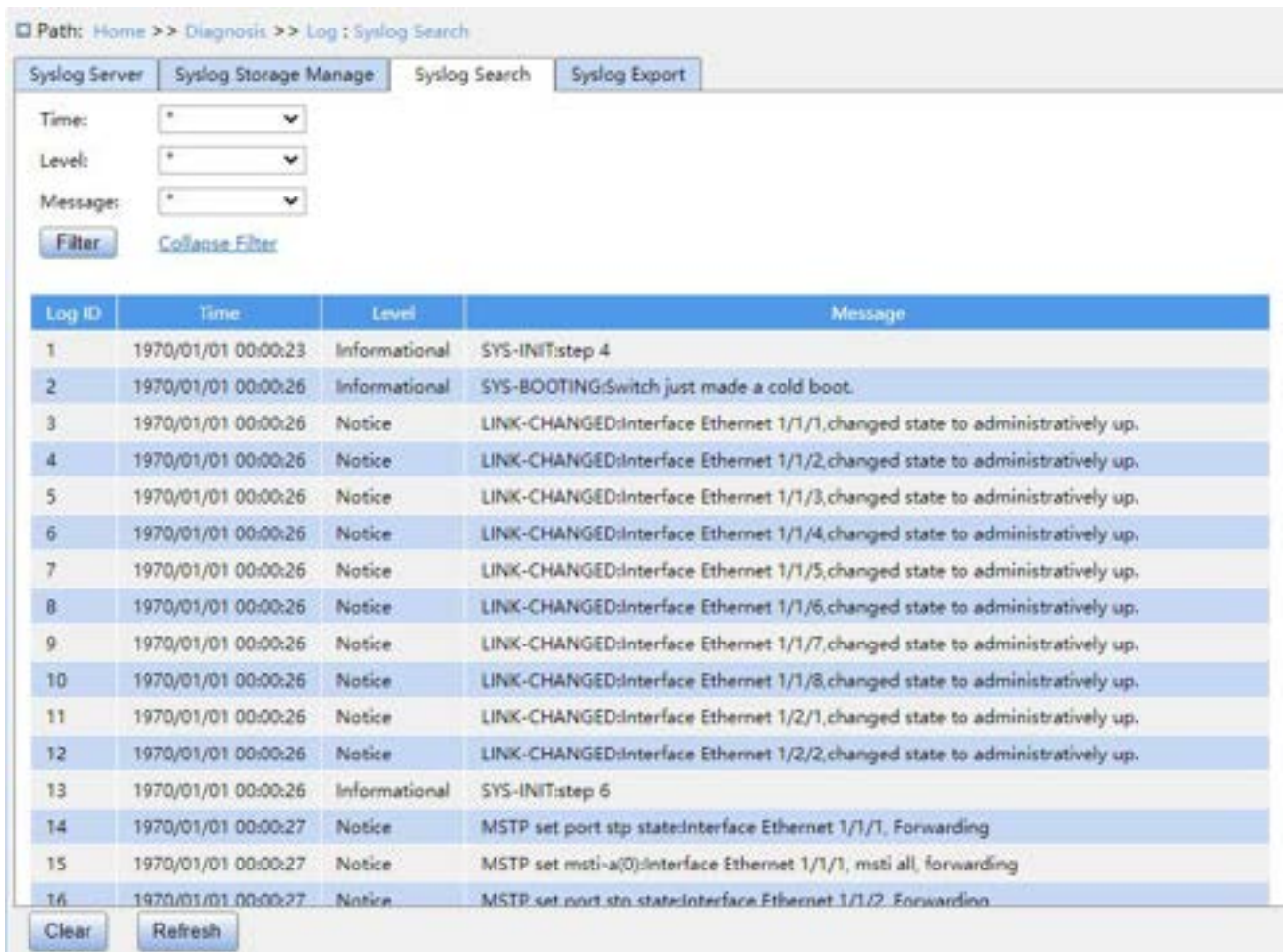
Figure 271 Syslog Search
