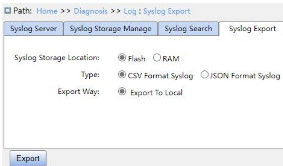
Figure 273 Log Export
