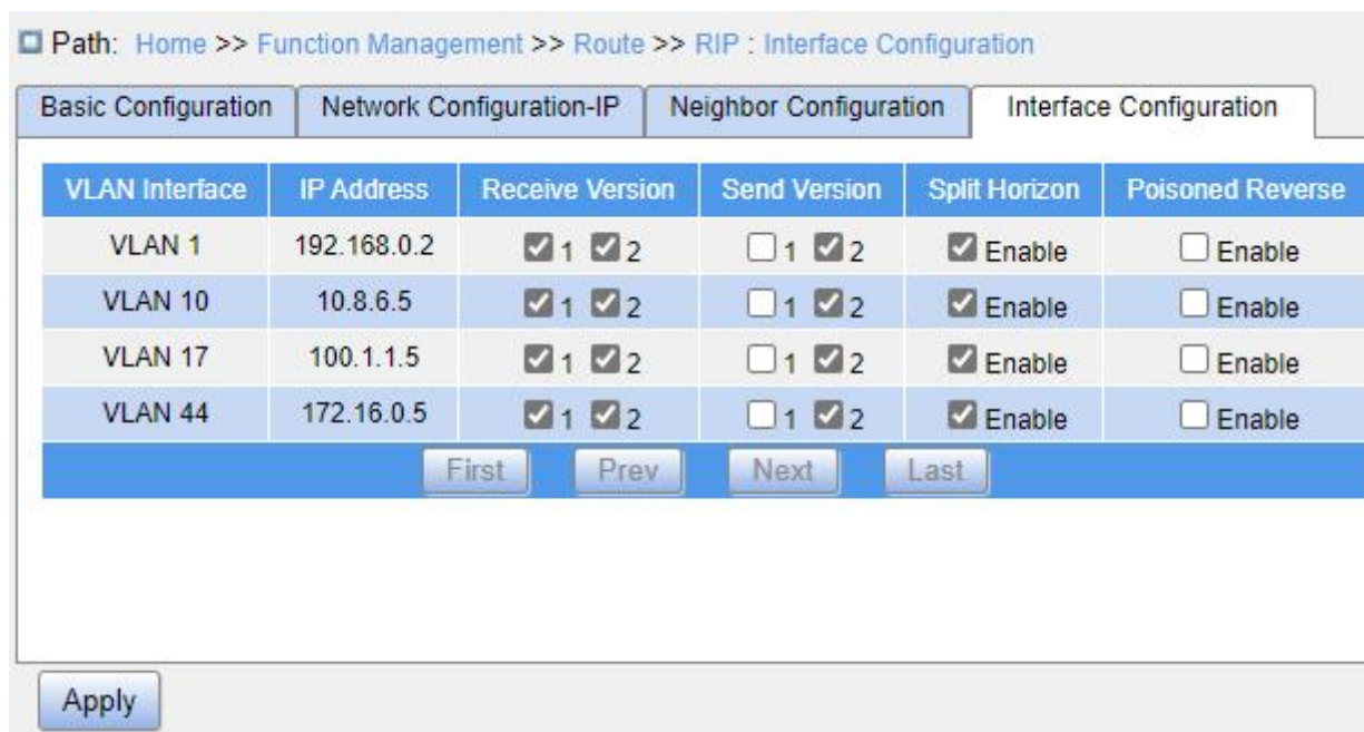
Figure 236 Interface Configuration
