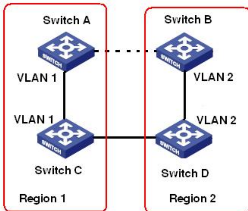
Figure 142 MSTP Topology
