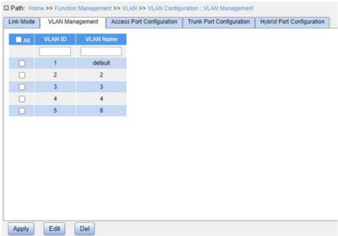
Figure 95 VLAN Management
