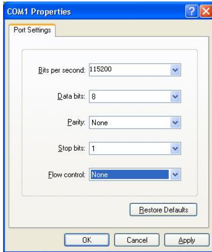
Figure 4 Set Port Parameters
