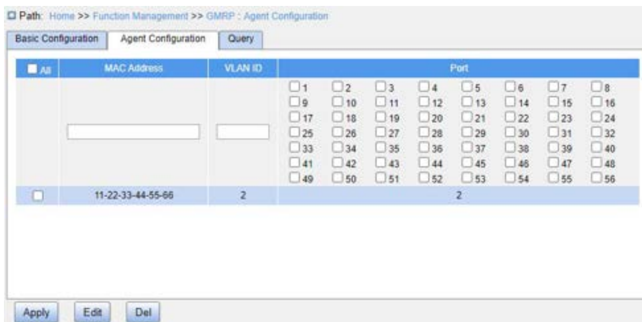
Figure 207 GMRP Agent Entry Configuration
