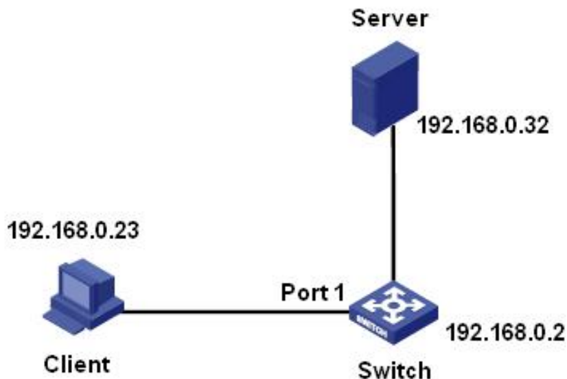
Figure 204 IEEE802.1x Configuration Example
