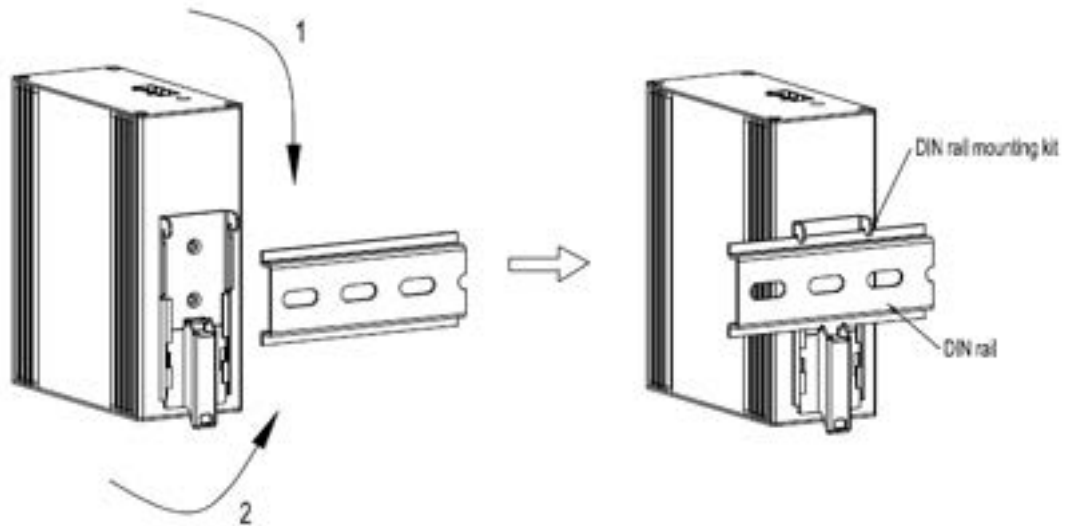
Figure 10 Opal5L-1SFP4T、Opal8L-2SFP6T DIN-Rail Mounting
