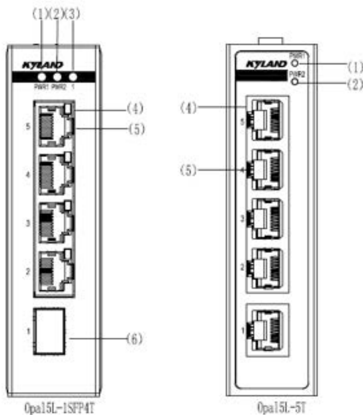
Figure 1 Opal5L Front Panel
