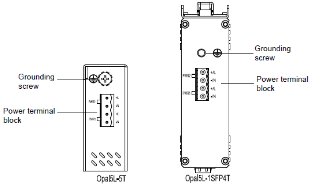
Figure 3 Opal5L Top Panel
