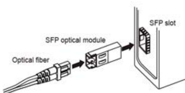
Figure 17 Connecting the 100M SFP Optical Module
