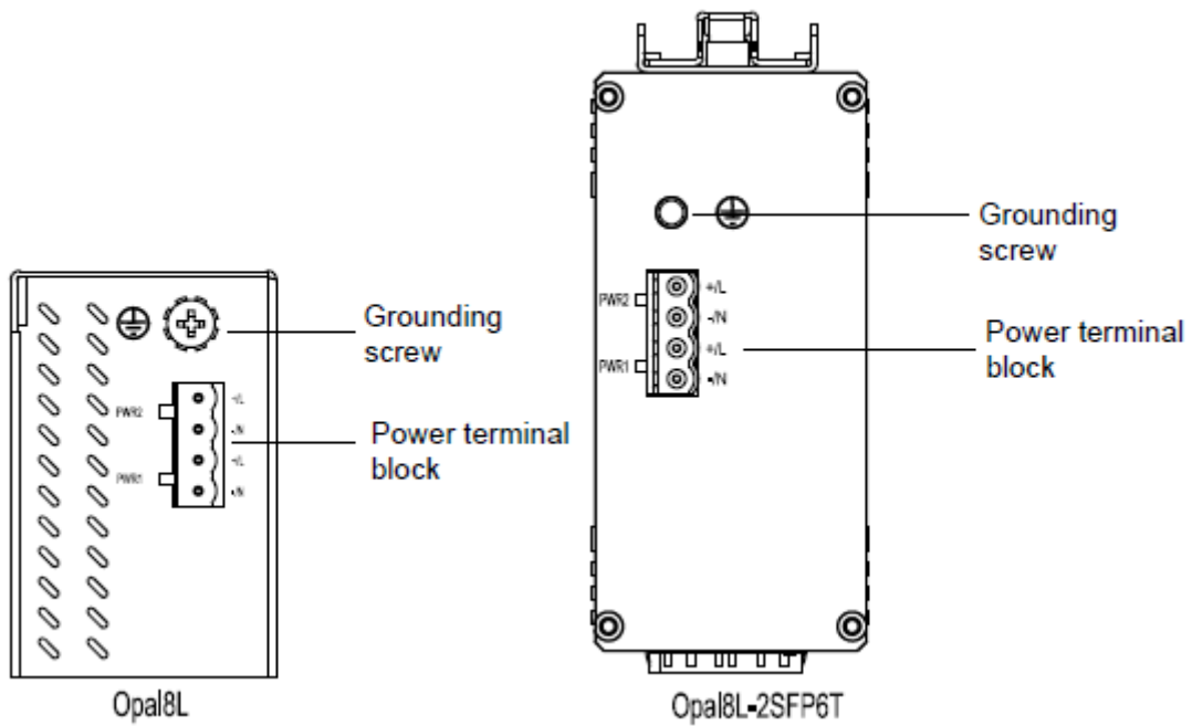
Figure 4 Opal8L Top Panel
