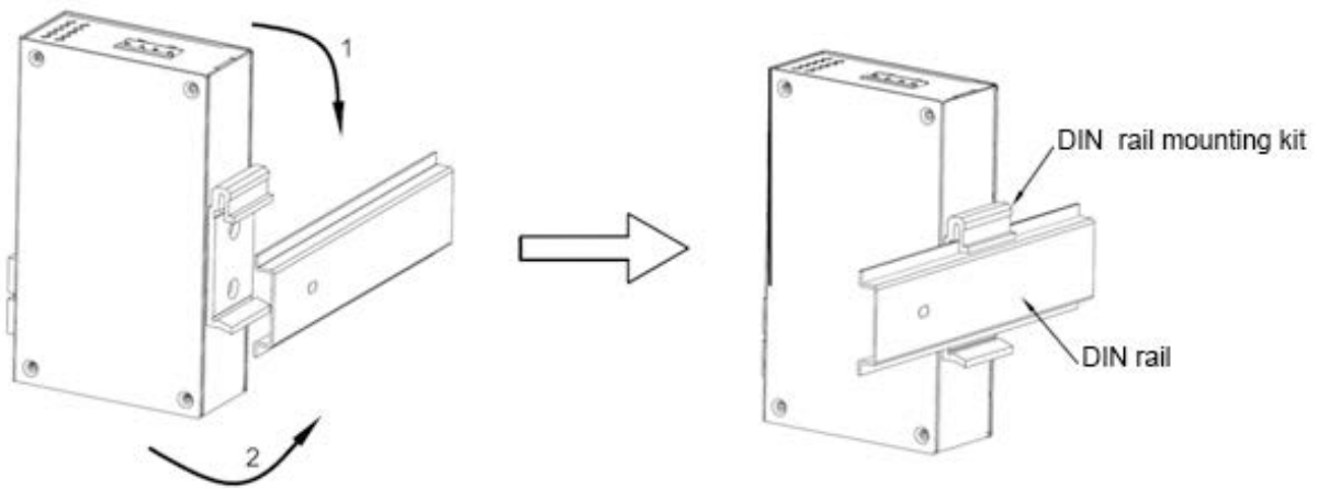
Figure 9 Opal5L-5T、Opal8L-8T DIN-Rail Mounting
