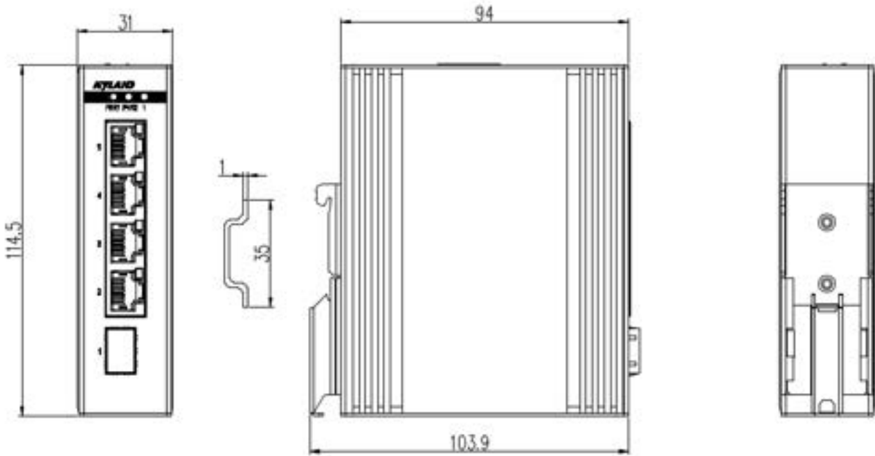
Figure 6 Opal5L-1SFP4T Dimensions for DIN-Rail Mounting (unit: mm)
