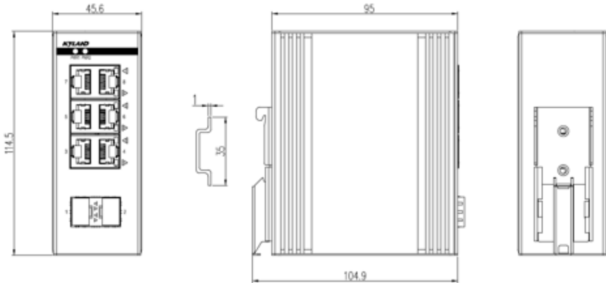
Figure 8 Opal8L-2SFP6T Dimensions for DIN-Rail Mounting (unit: mm)
