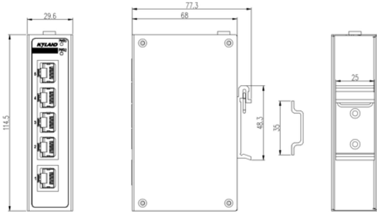
Figure 5 Opal5L-5T Dimensions for DIN-Rail Mounting (unit: mm)
