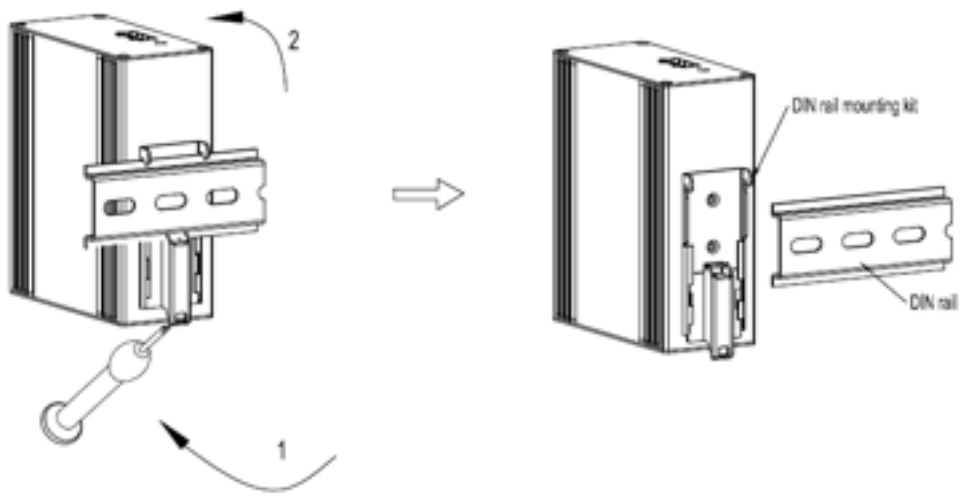
Figure 12 Opal5L-1SFP4T、Opal8L-2SFP6T DIN Rail Dismounting
