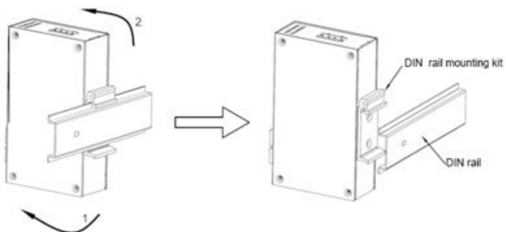
Figure 11 Opal5L-5T、Opal8L-8T DIN Rail Dismounting
