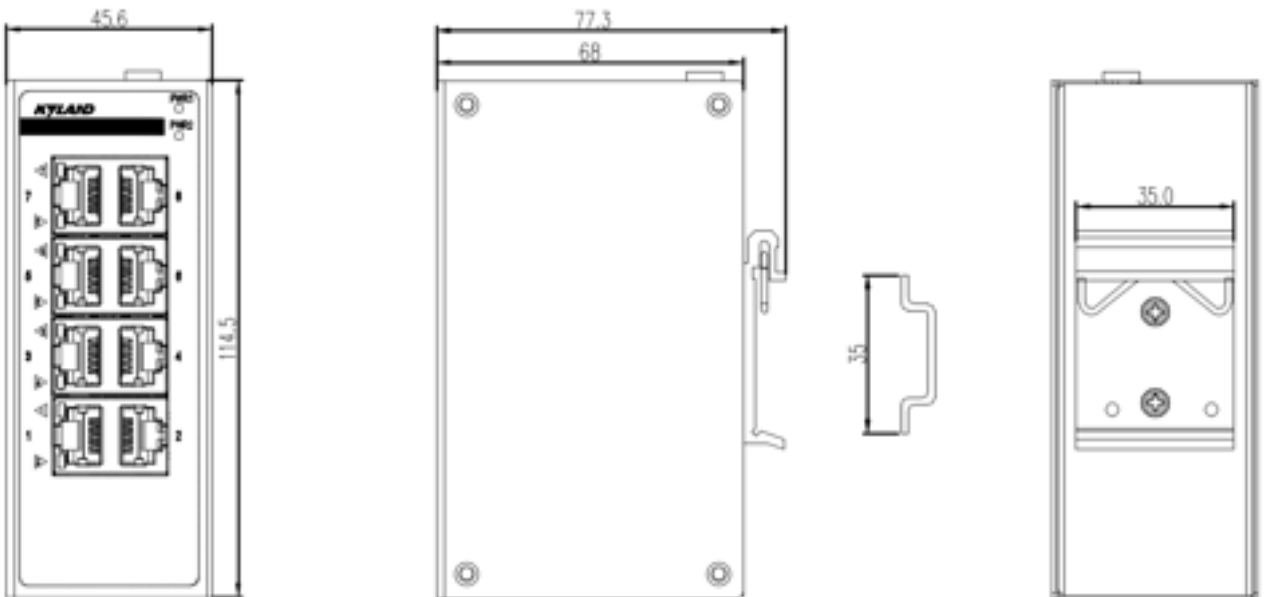
Figure 7 Opal8L-8T Dimensions for DIN-Rail Mounting (unit: mm)
