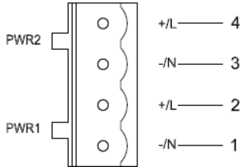
Figure 18 4-Pin 5.08mm-Spacing Plug-in Terminal Block (socket)
