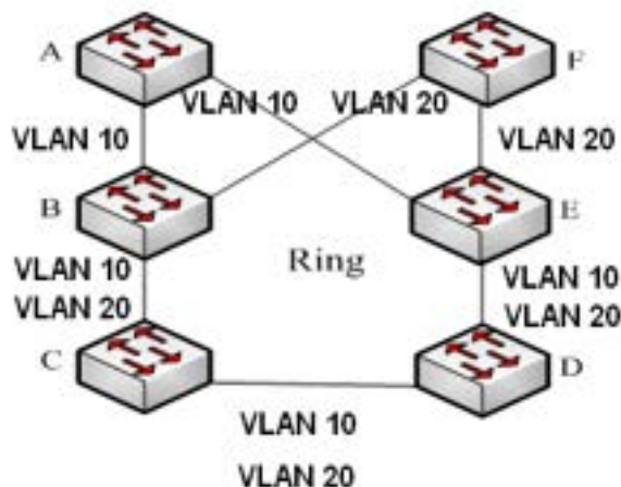
Figure 209 DT-Ring-VLAN
