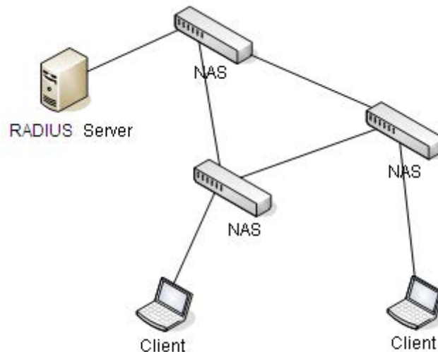
Figure 136 RADIUS Structure
