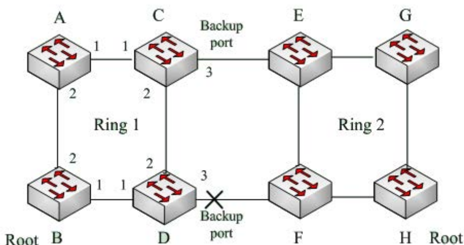
Figure 218 DRP Backup
