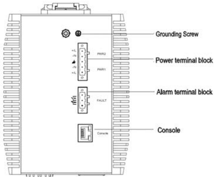
Figure 2 Low voltage products Top Panel
