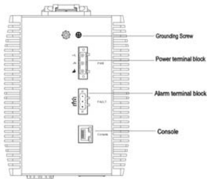
Figure 3 High voltage products Top Panel
