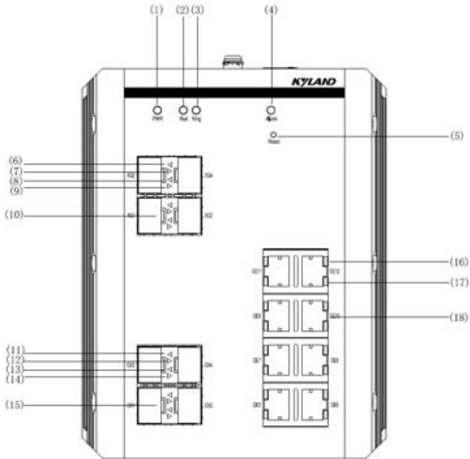
Figure 1 Front Panel
