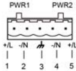
Figure 17 5-Pin 5.08mm-Spacing Plug-in Terminal Block
