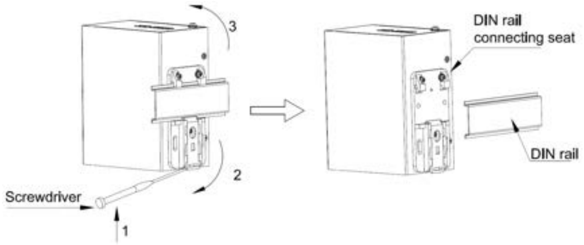
Figure 6 DIN-Rail 2 Dismounting
