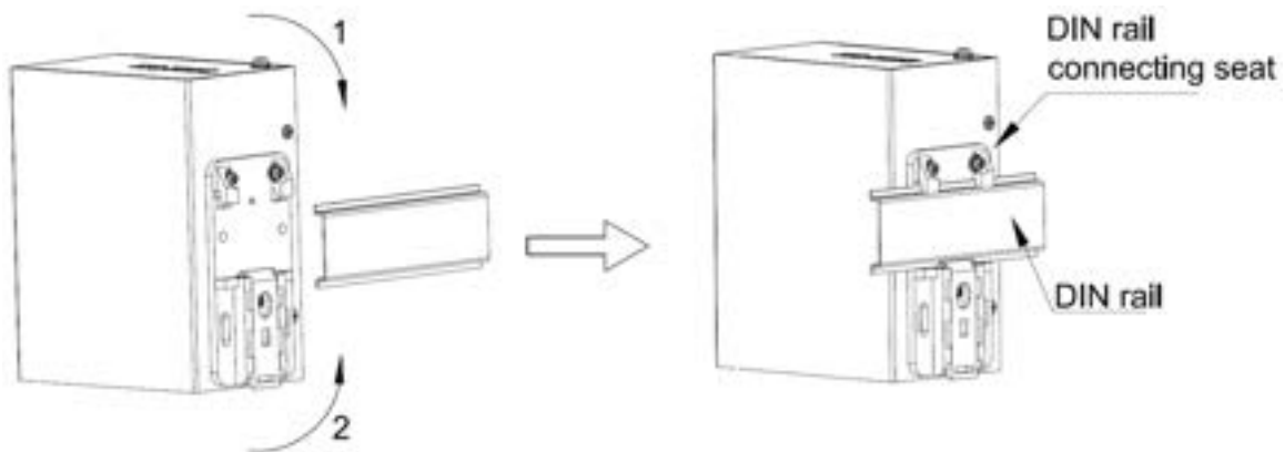
Figure 5 DIN-Rail 2 Mounting
