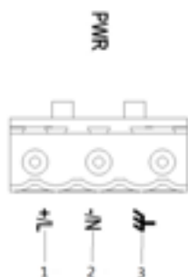
Figure 16 3-Pin 7.62mm-Spacing Plug-in Terminal Block (socket)
