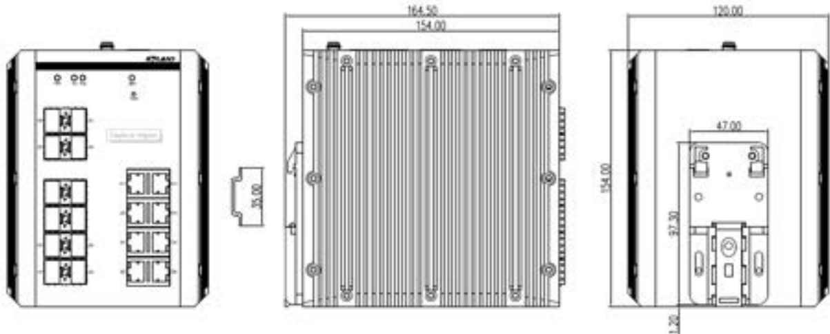
Figure 4 Dimensions for DIN-Rail Mounting (unit: mm)
