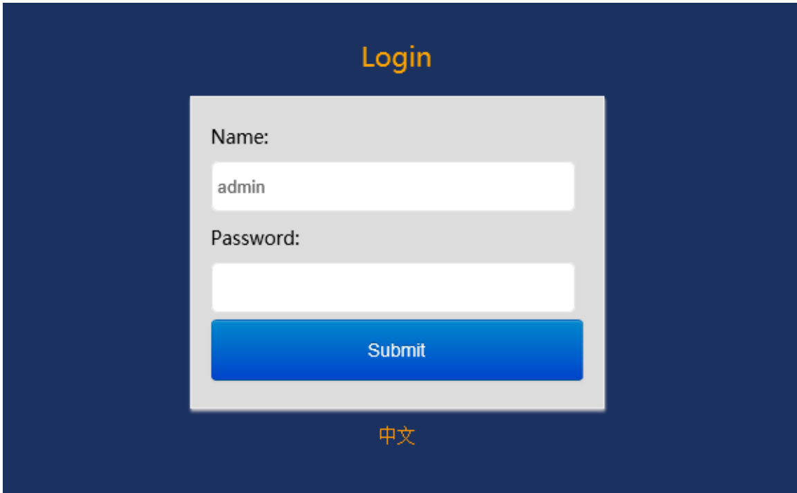
Figure 3 Login Screen
