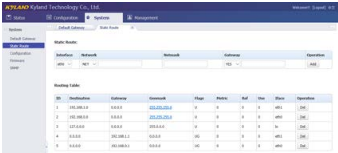
Figure 22 Route Screen
