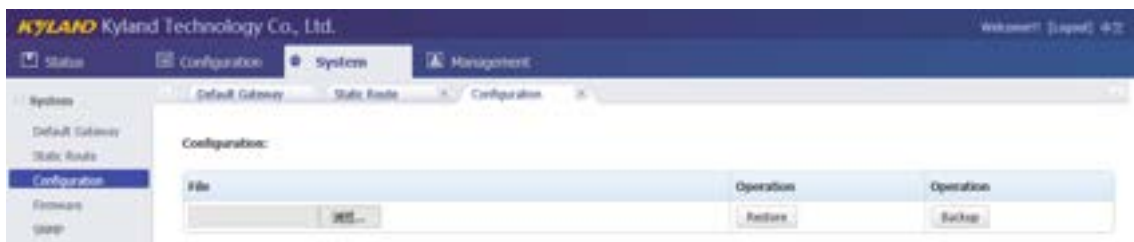
Figure 23 Configuration Screen
