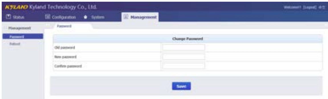
Figure 26 Management Screen
