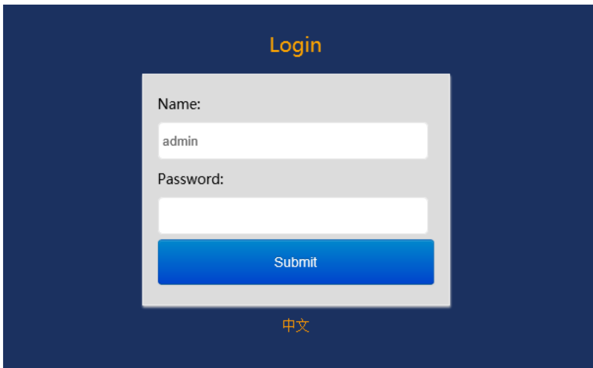
Figure 5 Login Screen
