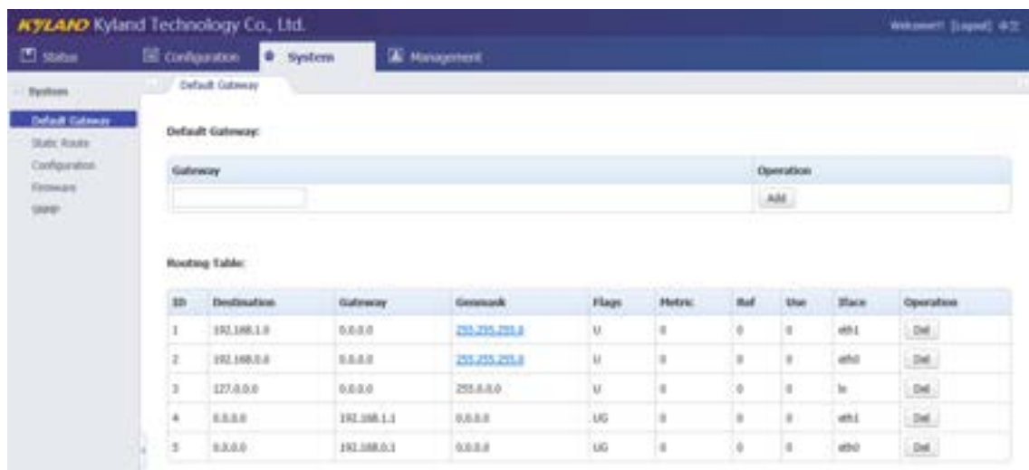
Figure 21 System Screen
