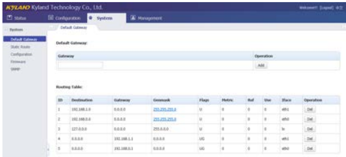
Figure 20 System Screen
