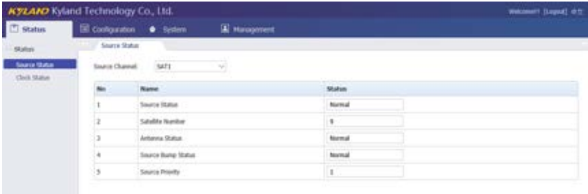
Figure 7 Status Screen
