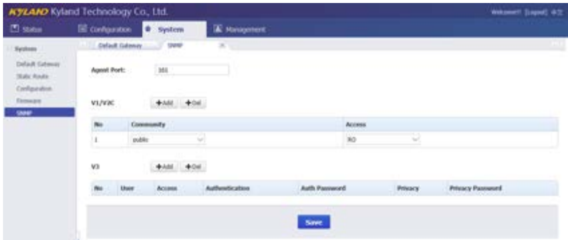
Figure 25 SNMP Screen
