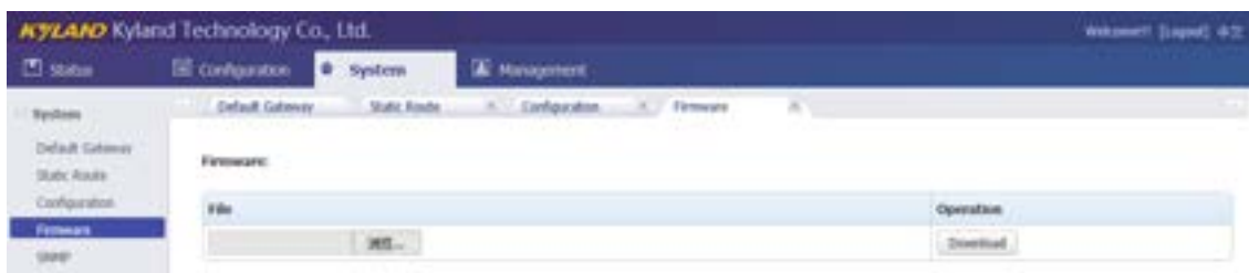
Figure 24 Firmware Screen
